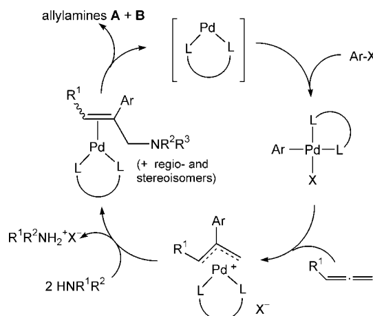
Scheme 2. Anticipated reactions for a three-component intermolecular carbopalladation-amination of allenes to give allylamines.
