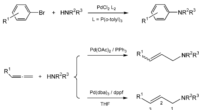
Scheme 1. Selected transition metal-catalyzed C–N coupling reactions.
